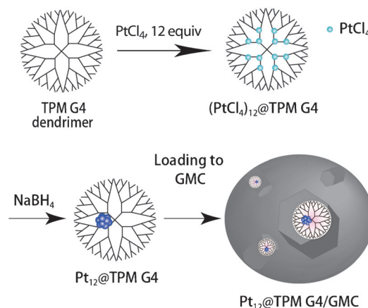
Scheme 1. Representation of Pt 12 @TPM G4/GMC using a phenylazomethine dendrimer. GMC = graphitized mesoporous carbon.
